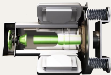
Inverter Linear Compressor - Two Step Coil Control
