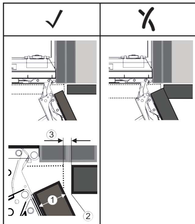
Fig. 68 (1) Front thickness (FD) (2) Edge radius (R) (3) Clearance (S)
