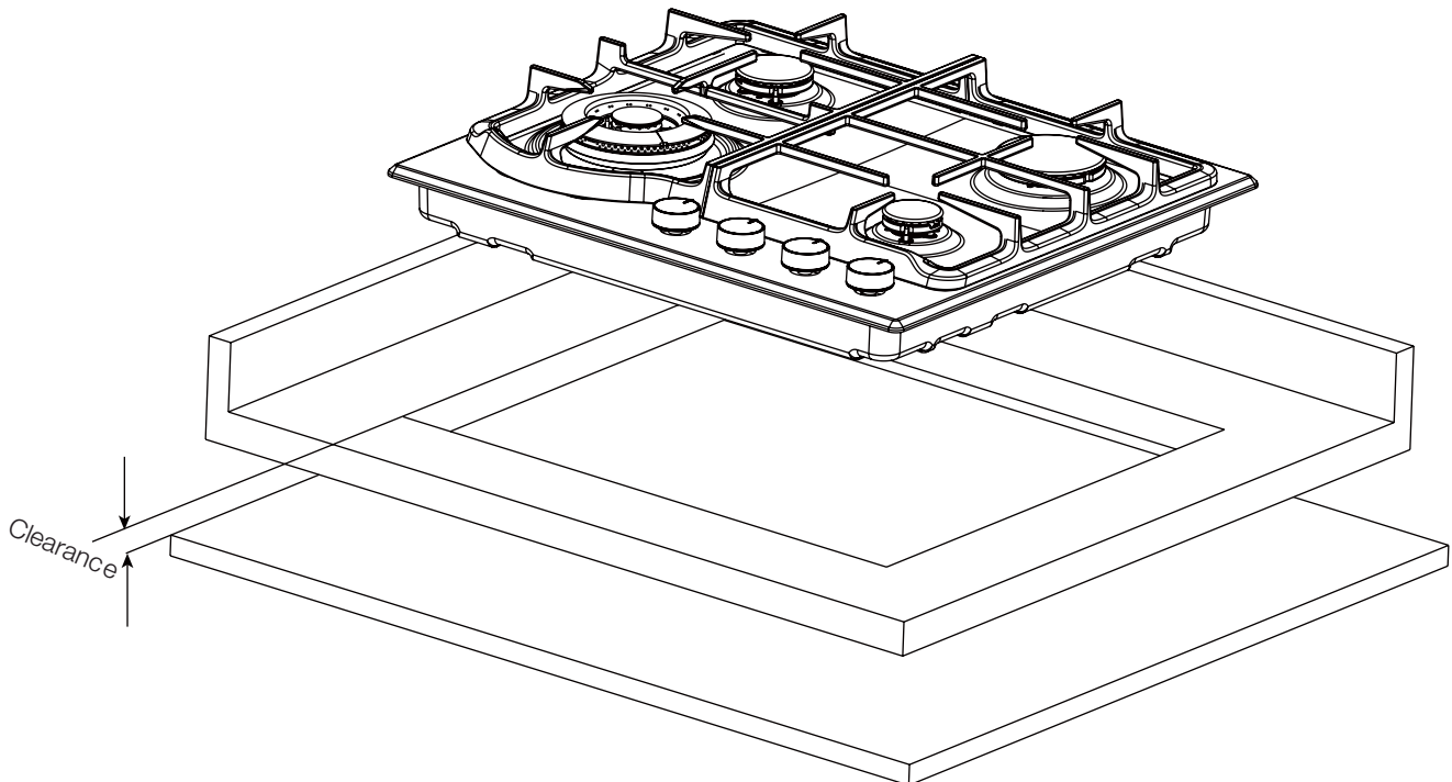
Figure 5c – Clearance from bench to bottom
