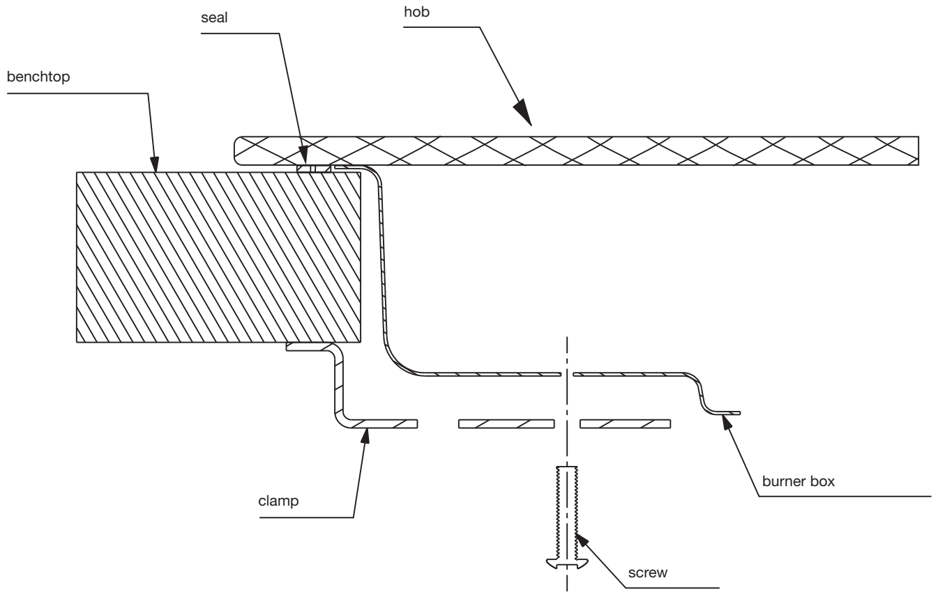
Figure 7 – Clamp fitment
