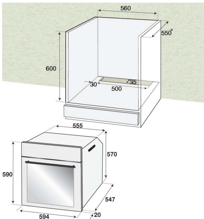
Cabinet Dimensions
